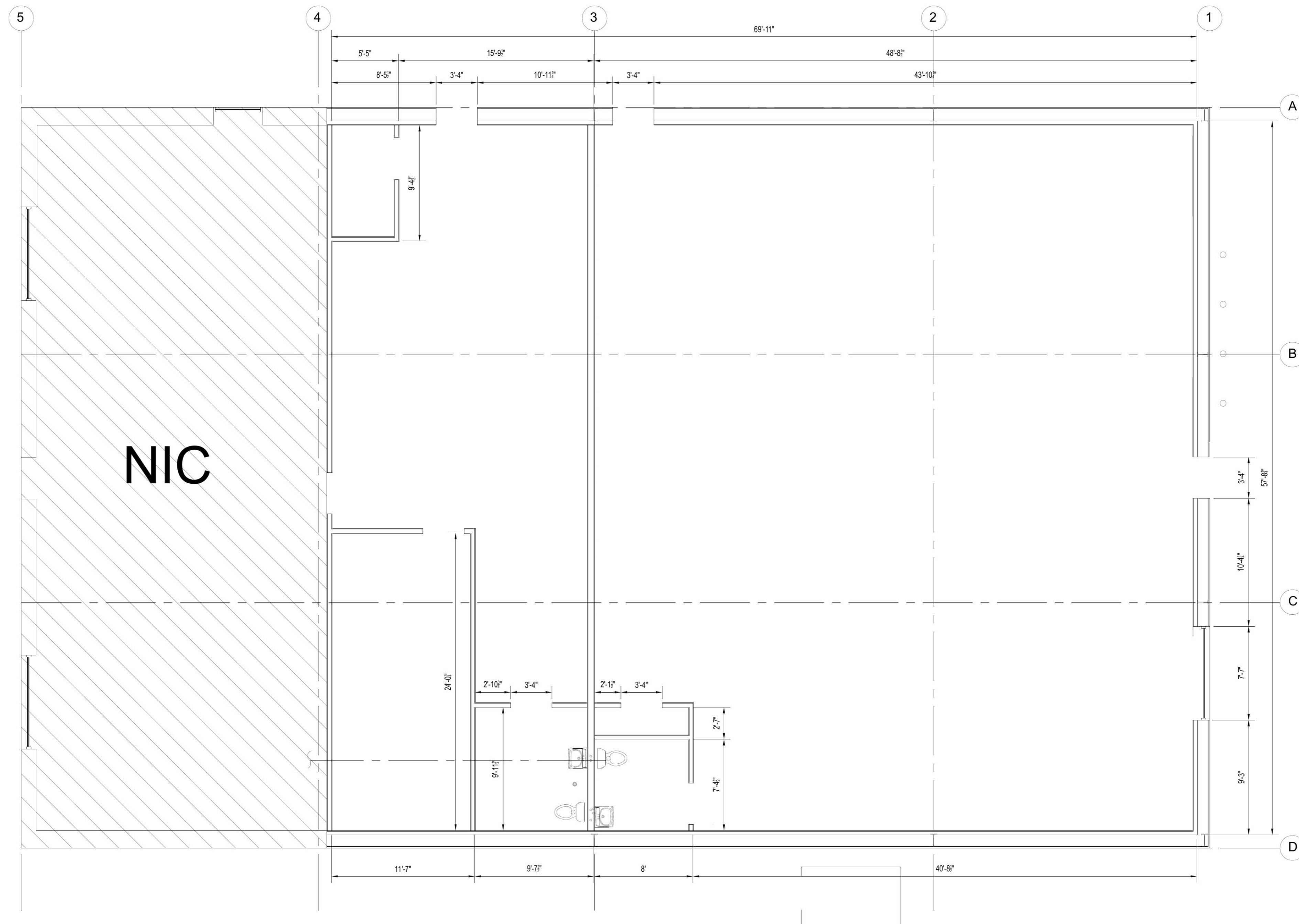
DIMENSIONAL PLAN SCALE: 3/16" = 1'-0"
