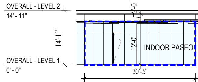
3 PASEO ELEVATION - RETAIL R07 LOD SCALE: 1/16" = 1'-0"
