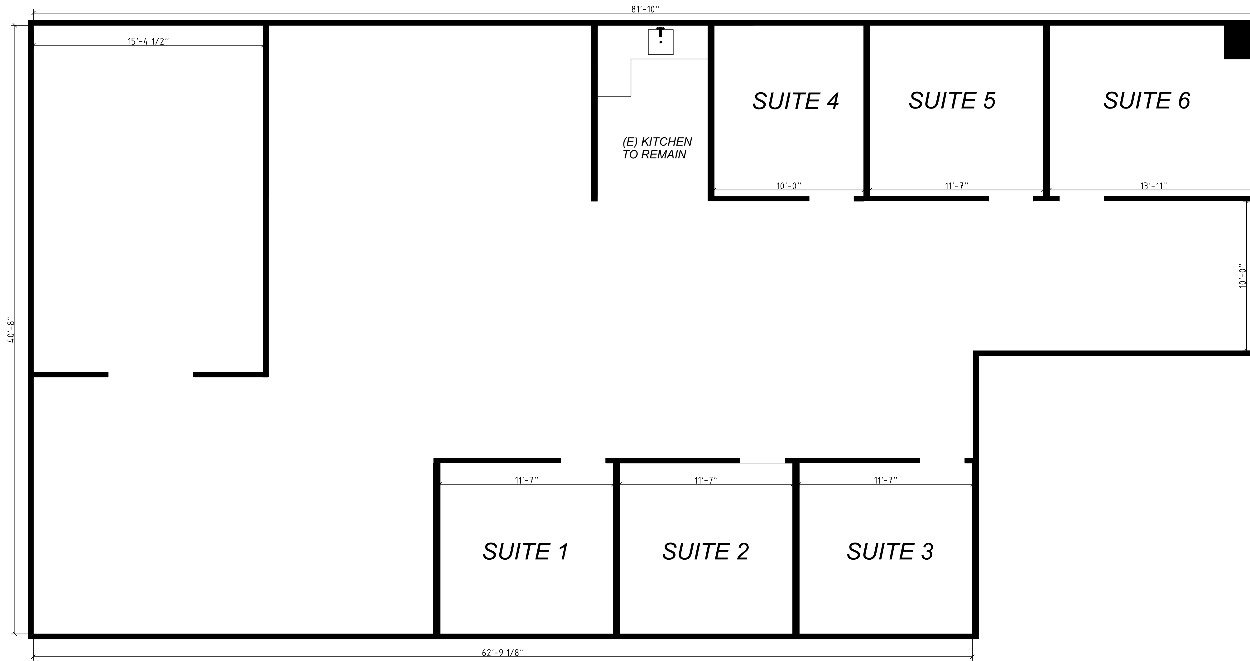
1 FLOOR PLAN A-7 1/4"=1'-0"
