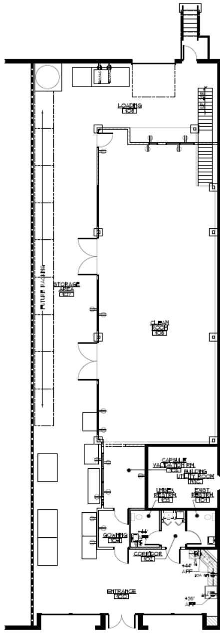
1511 Wayside Road, Tinton Falls Current As-Built Plan Warehouse Space #6 – 4,728 Rentable SF
