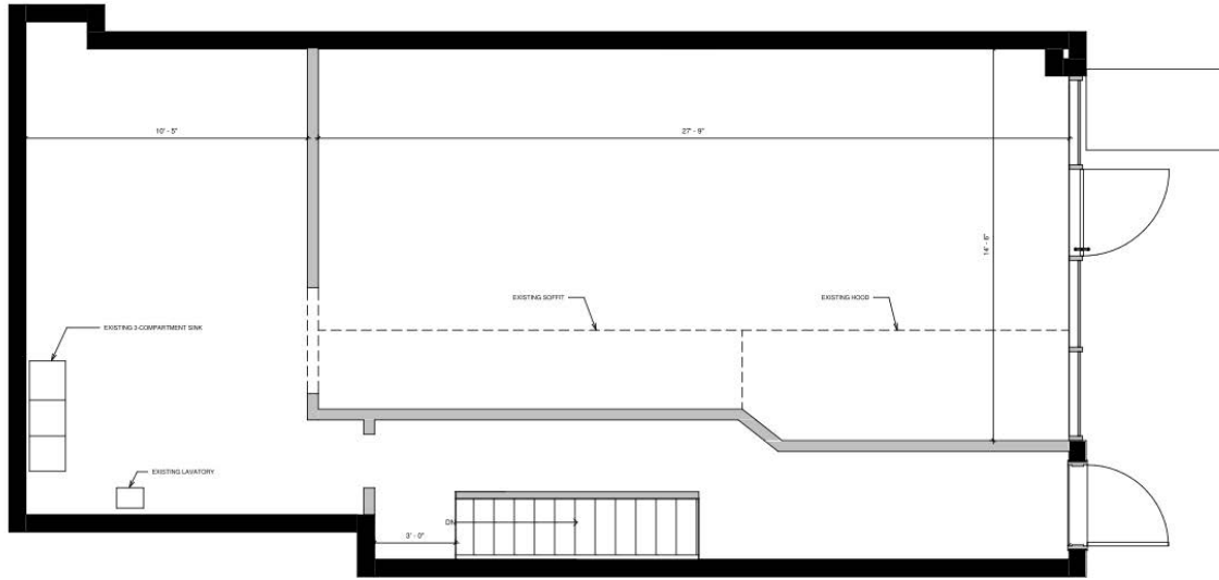
1 EXISTING GROUND FLOOR PLAN
