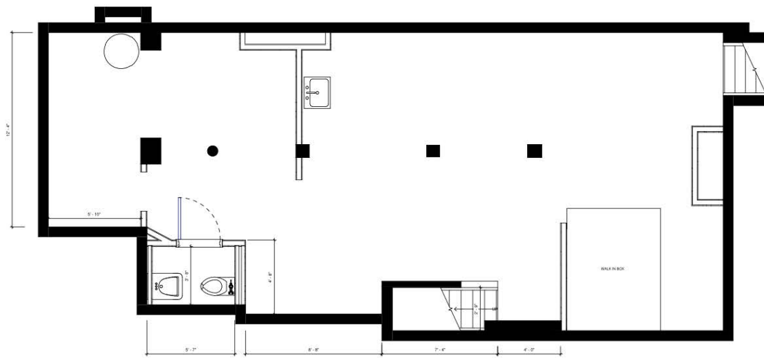
2 EXISTING CELLAR PLAN
