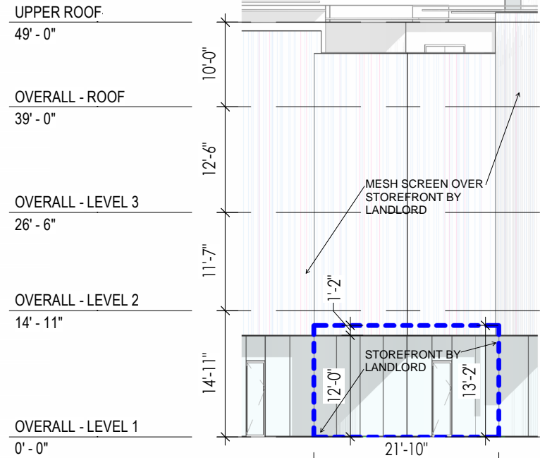
3 SOUTH ELEVATION - RETAIL R12 SCALE: 1/16" = 1'-0"
