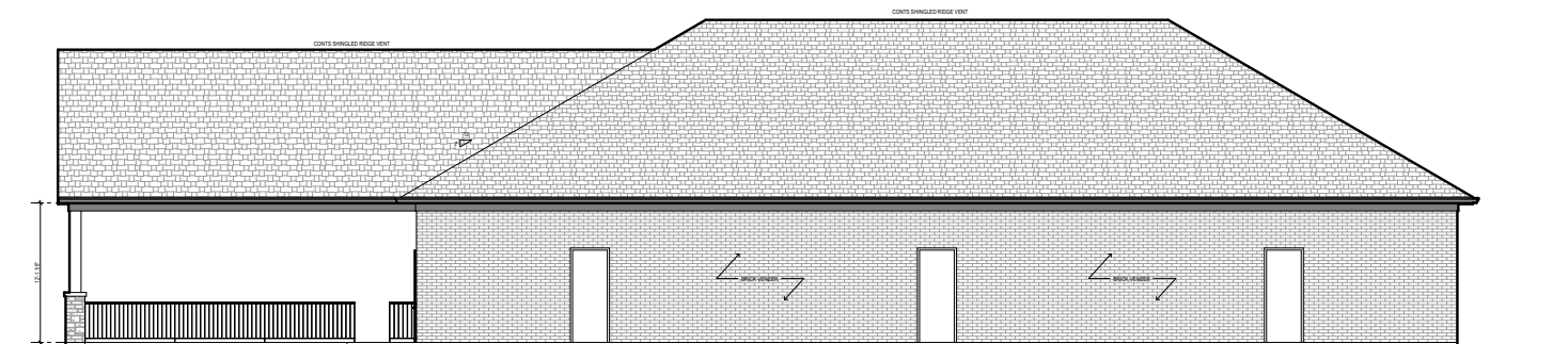
2 A-1 East Elevation SCALE: 3/16" = 1'-0"
