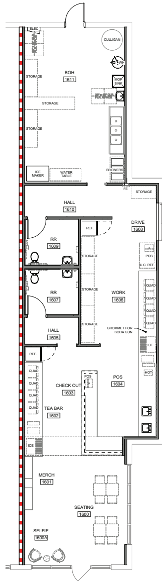
① FURNITURE PLAN 1/4" = 1'-0"
