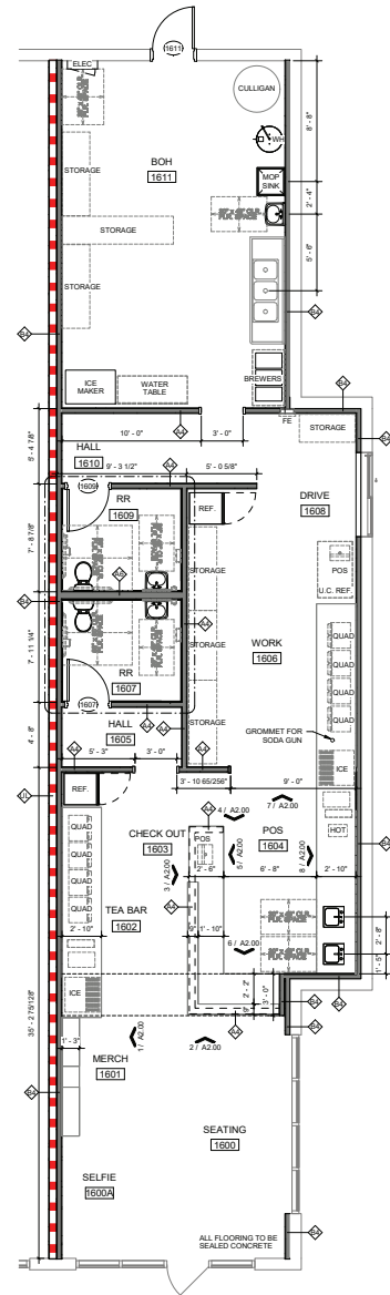
③ FLOOR PLAN 1/4" = 1'-0"
