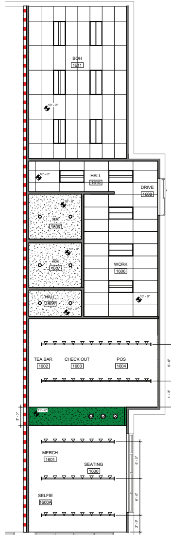
② REFLECTED CEILING PLAN 1/4" = 1'-0"
