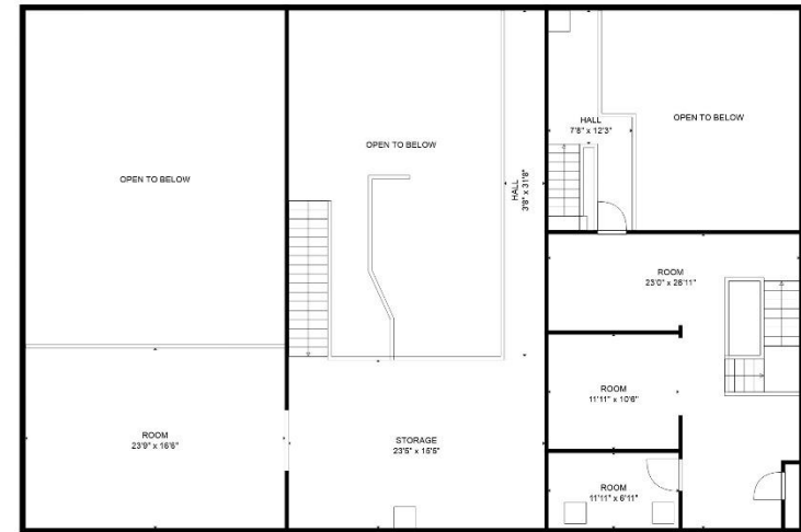
FLOOR 2
